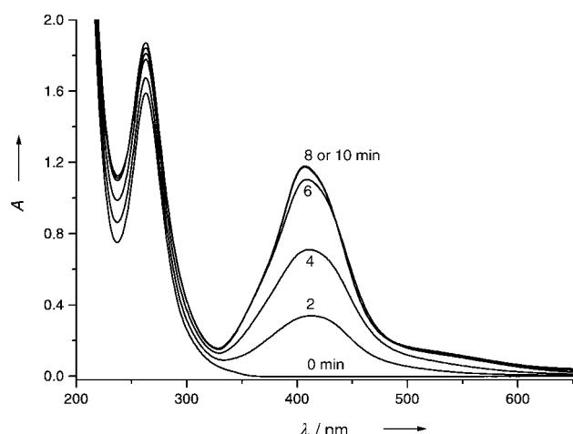
Figure 6. Photolysis profile: the formation of colloidal silver at different illumination times ( \lambda \approx 410 nm) and the stability of [\text{SiW}_{12}\text{O}_{40}]^{4-} photocatalyst ( \lambda = 263 nm). Photolysis of a deaerated solution containing propan-2-ol (0.5 M), [\text{SiW}_{12}\text{O}_{40}]^{4-} (0.035 mM), \text{Ag}^+ (0.1 mM) at pH 5 ( \lambda > 320 nm).
